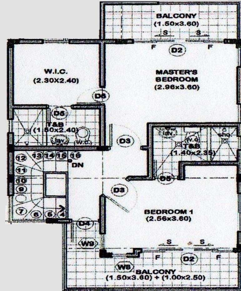
2 ND FLOOR
